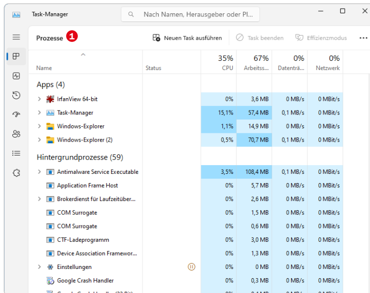
Task-Manager
