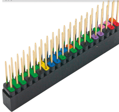
Figure 1.4: Colored header.
