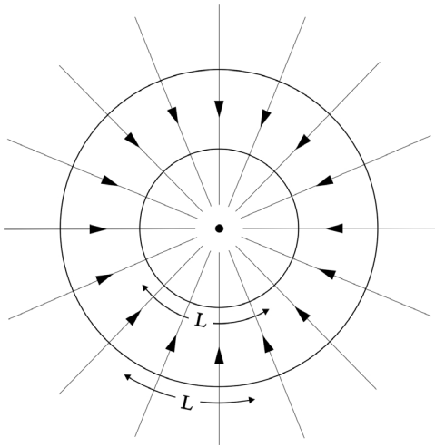
Figure 1.1 Lines of force from an infinite line source (viewed end on). The distance between the lines increases linearly with distance from the source so that an arc of the inner circle of length L is cut by four lines but an arc of the same length on the outer circle, with double the radius, is cut by only two.
