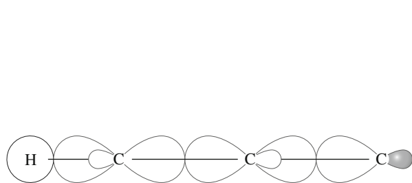
\sigma -Bindungen
