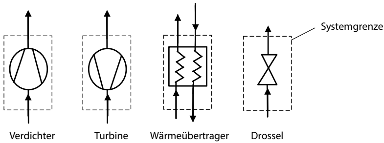
Abb. 2.3 Offene Systeme.
